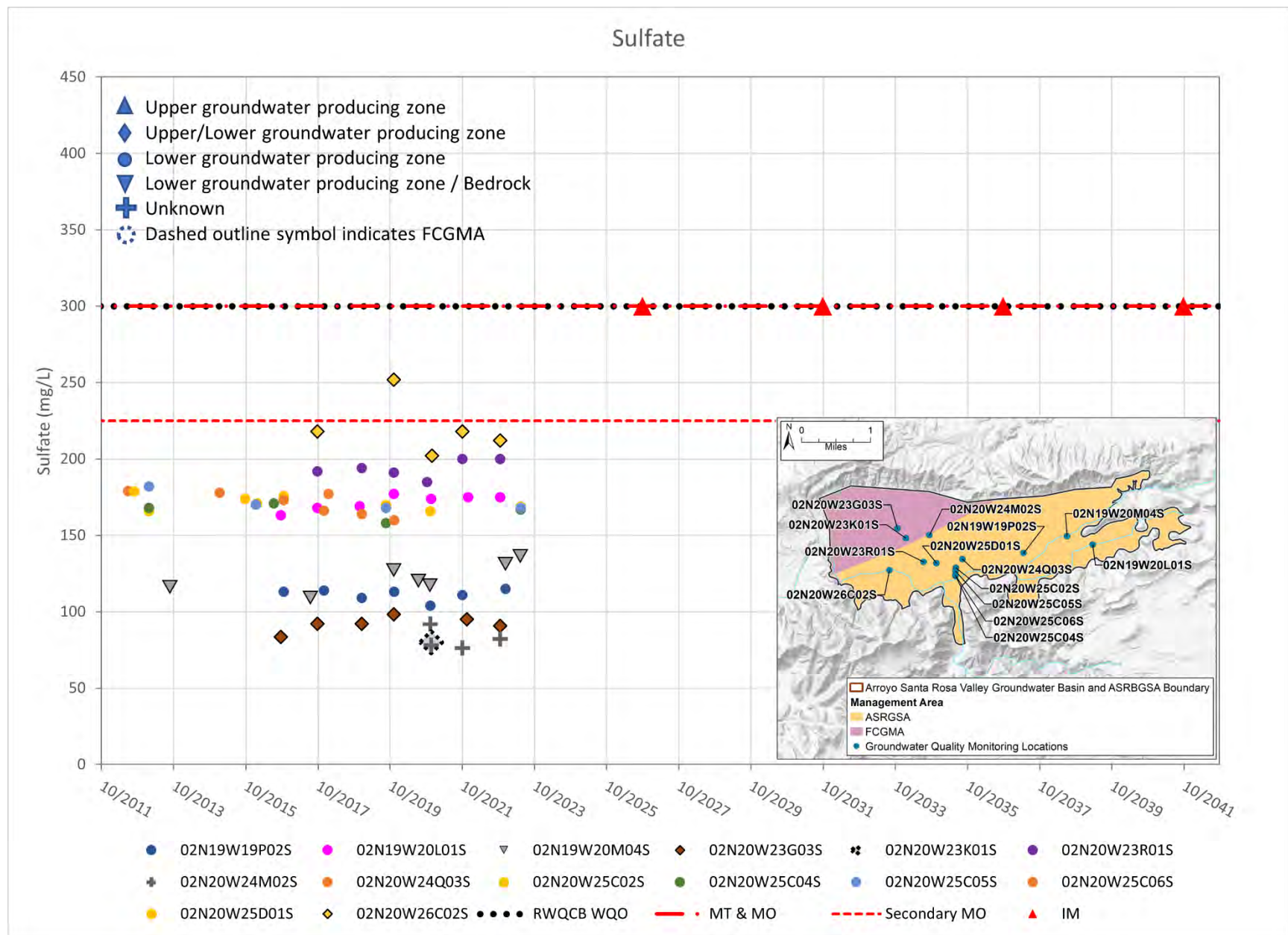
Figure 3.5d Sulfate Chemograph with Minimum Thresholds, Measurable Objectives, and Interim Milestones, Water Years 2022-2023.
